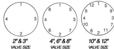
TORQUE SEQUENCE FOR ANSI CLASS 150 FLANGES
